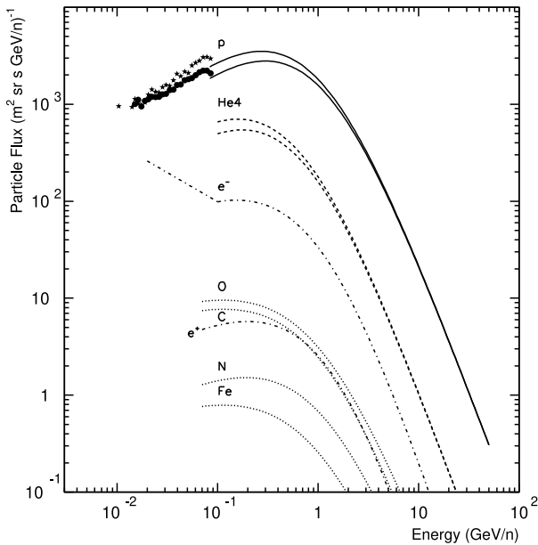
Fig. 2. Predictions of cosmic-ray energy spectra after the Solar Orbiter launch. The top and bottom continuous (protons) and dashed ( 4 He nuclei) curves are obtained with the G&A model above 70 MeV/n for minimum and maximum solar modulation parameter values of 300 MV/c and 340 MV/c, respectively. Maximum ( \phi=300 MV/c) and minimum ( \phi=340 MV/c) proton and helium predictions apply to years 2020 and 2022, respectively. The dot-dashed (dotted) curves indicate the electron and positron (nucleus) energy spectra at solar minimum.
